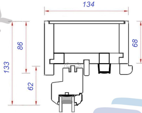
Section A-A with VENTILATION
