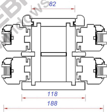
Section B-B SOLID MULLION
